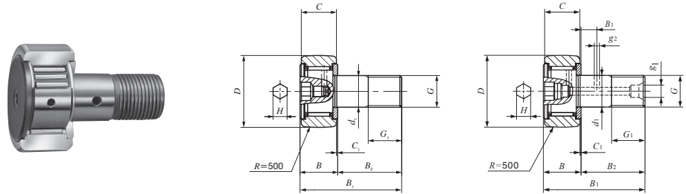
CF...WBR Stud dia. d_1 3-10mm
